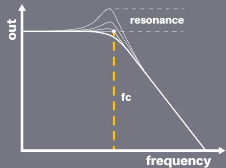
Fig.3 Low Pass Filter
